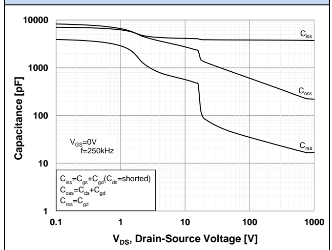
Figure 12. Capacitance Characteristics
