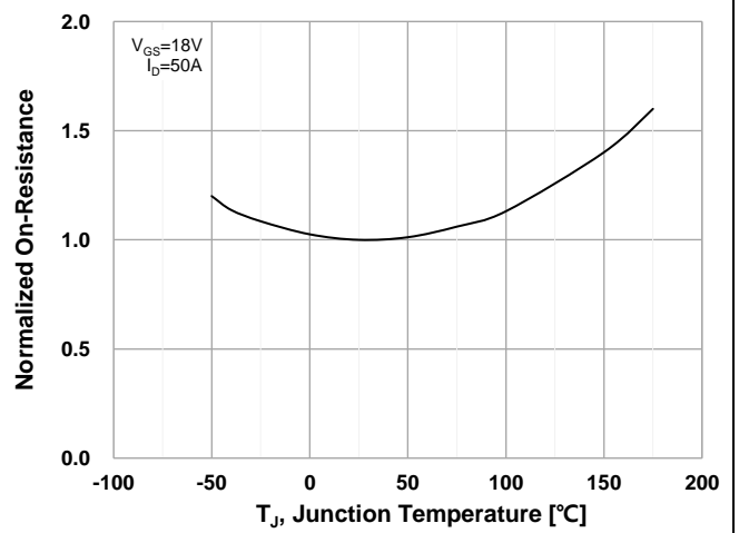
Figure 4. Normalized On-Region Characteristics vs. Temperature
