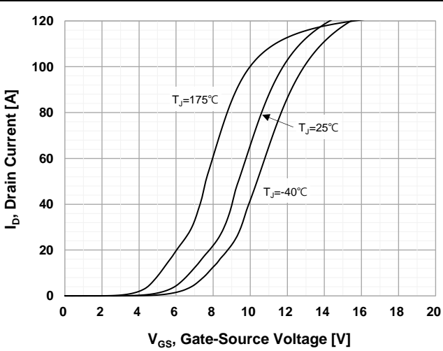
Figure 5. Transfer Characteristics
