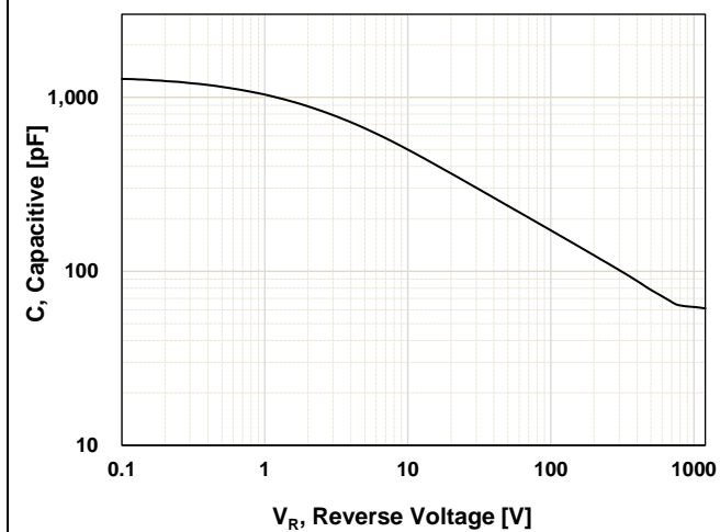
Figure 7. Capacitive Characteristics
