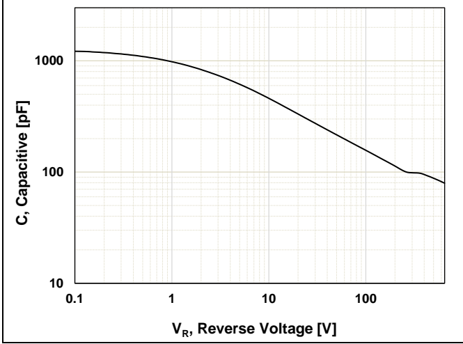
Figure 7. Capacitive Characteristics
